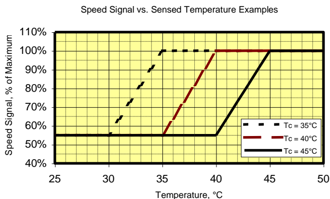
Chart 1.0: Fan speed signal vs. sensor temperature (5deg slope).
