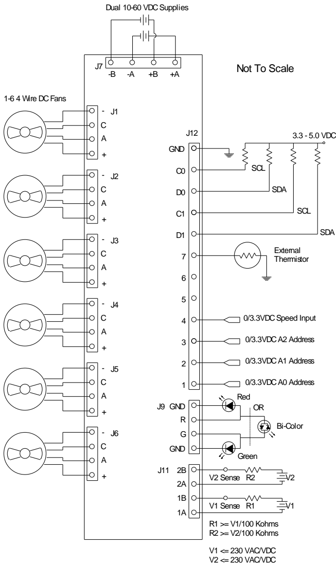
FIGURE 1.0: Connection diagram showing input power, fan, interface, temperature sensor, LEDs and alarm connections for a Cirrus-6 Fan Control.
